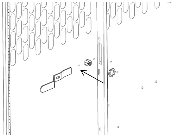
Viewed from cargo compartment
